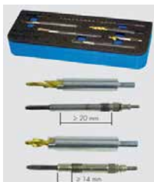
Urborningsats M10x1 M10x1,25 GO474
